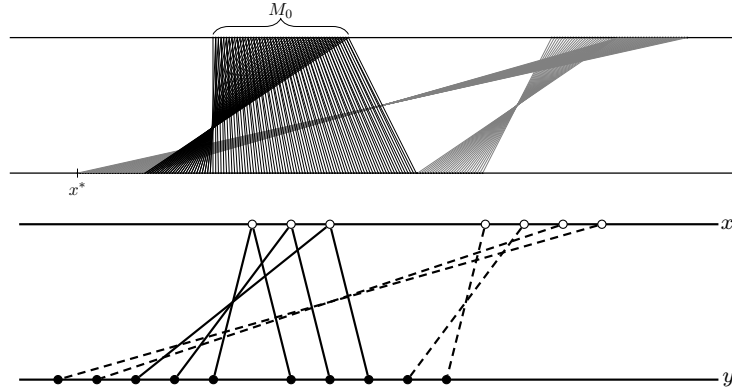
FIGURE 1. Simulations of the Increasing Supermartingale Transport. We observe an interval of Left-Curtain kernels (black/continuous) on the left and an interval of antitone kernels (gray/dashed) on the right. The destinations of the right interval are on both sides of the destinations of the left one. (The definitions of x^* and M are given in Sections 3 and 5, respectively.)
