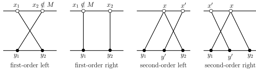
FIGURE 3. Forbidden configurations in the monotonicity properties
