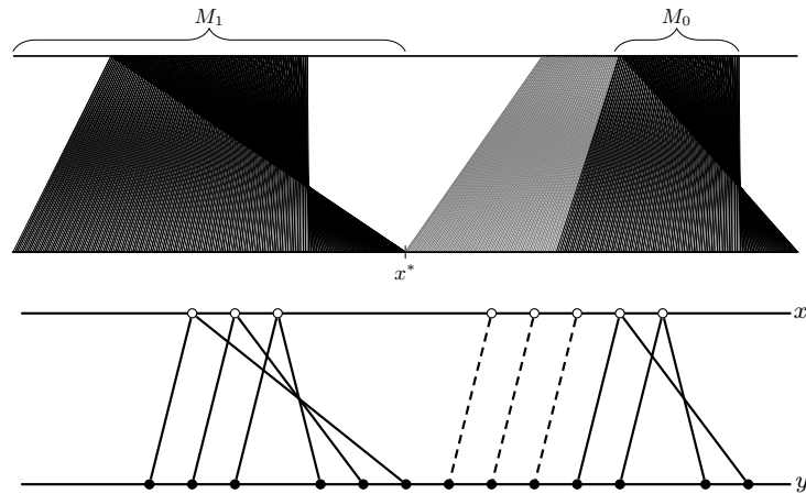
FIGURE 2. Simulations of the Decreasing Supermartingale Transport. We observe an interval of Right-Curtain kernels on the left, followed by an interval of Hoeffding–Fréchet kernels and another interval of Right-Curtain kernels. The destinations of these intervals preserve the original order.
