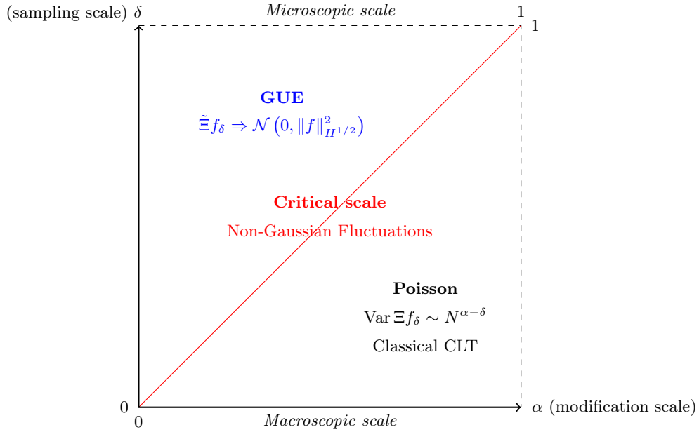
FIG 1. Diagram of the fluctuations for a smooth linear statistics of a Modified GUE as a function of the scale \delta and the modification scale \alpha .
